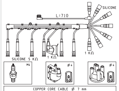
COPPER CORE CABLE \varnothing 7 mm
