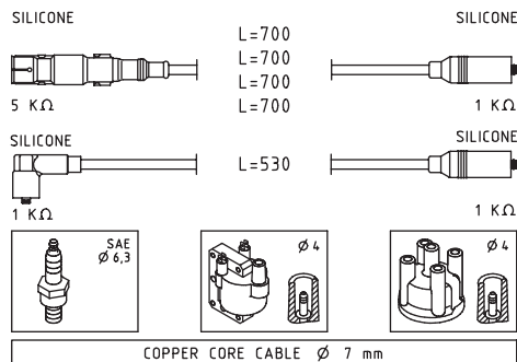
COPPER CORE CABLE \varnothing 7 mm
