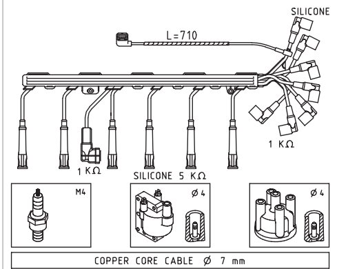
COPPER CORE CABLE \varnothing 7 mm
