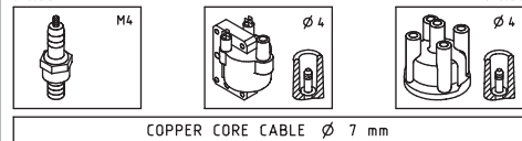
COPPER CORE CABLE Ø 7 mm
