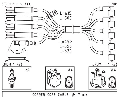
COPPER CORE CABLE \varnothing 7 mm
