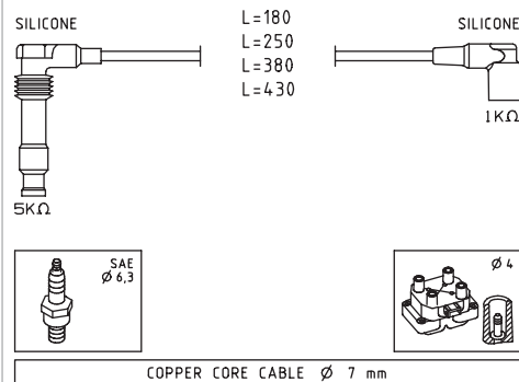
COPPER CORE CABLE \varnothing 7 mm
