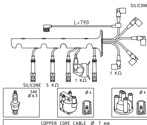
COPPER CORE CABLE \varnothing 7 mm
